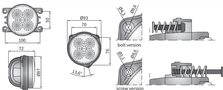
Lamp positioning: 8° from the vertical for light distribution angle 58°, h=2,5m 12° from the vertical for light distribution angle 35°, h=2,5m
